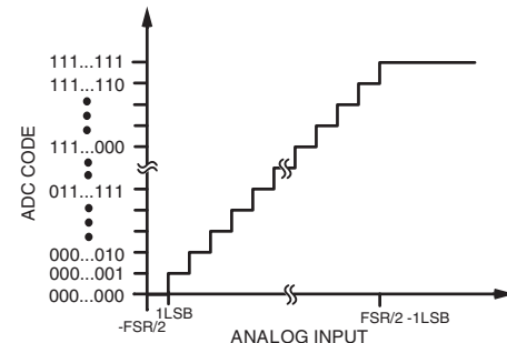
Figure 9. Straight Binary Transfer Characteristic (Bipolar Ranges)
