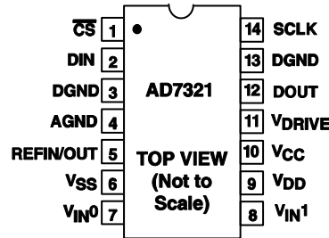
Figure 3. AD7321 Pin Configuration TSSOP
