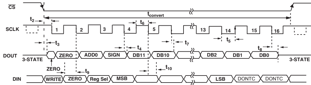
Figure 14. Serial Interface timing Diagram (Control register write)
