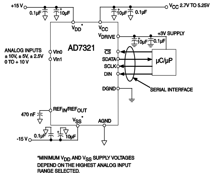
Figure 12. Typical Connection Diagram
